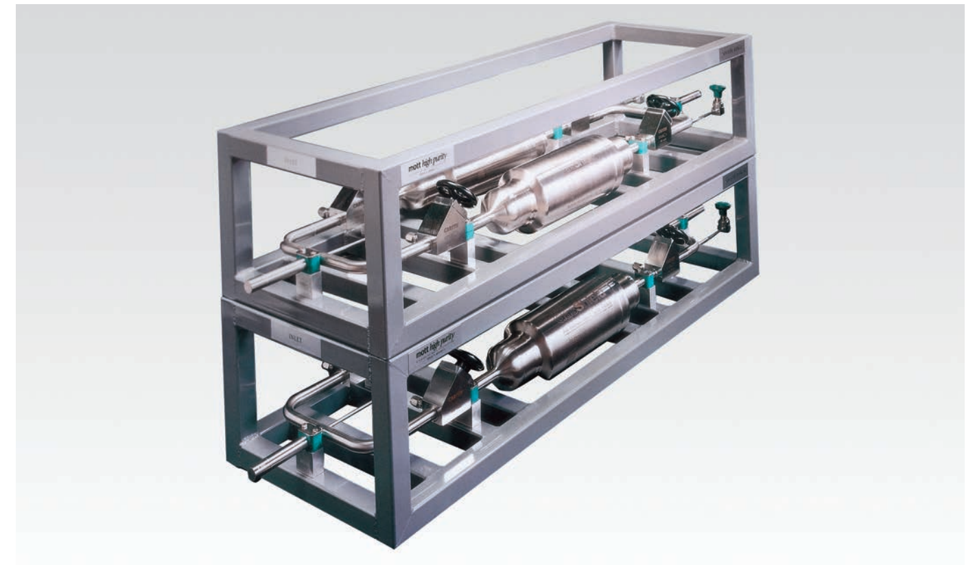
The supporting skids which include the ancillary tubing, iso-kinetic ports, isolation valves, pressure gauges and skid supports can be supplied by Mott Corporation or are supplied by third party fabricators.
