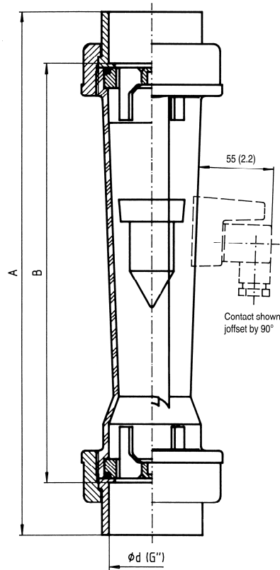
Fig. 4 FVA Troglux short version, dimensions in mm
