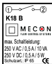
Fig.6 Contact K 18 B
