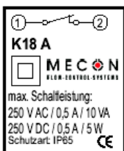
Fig.5 Contact K 18 A
